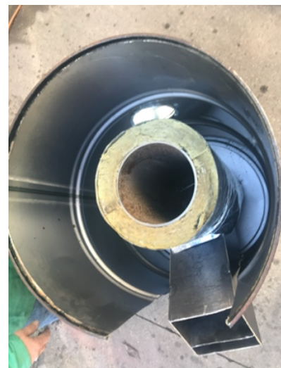
Figure 2 – Insulated Chimney
